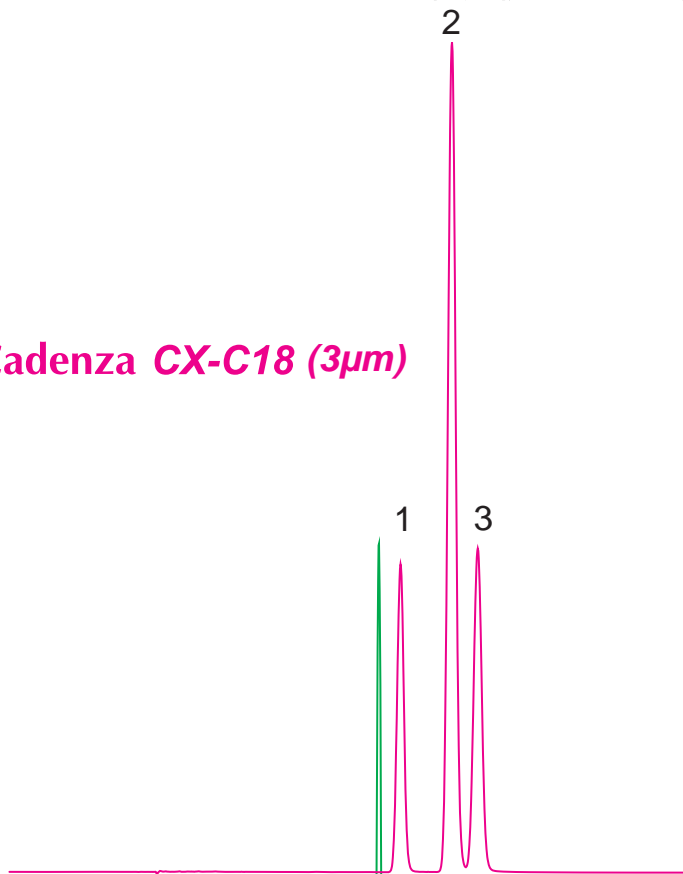
2 m -terphenyl
